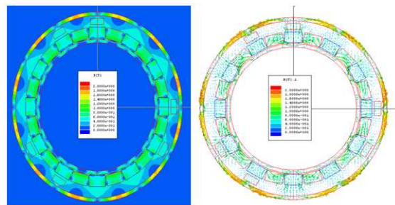
Fig. 9: Flux Distribution of the machine (FE Results)
